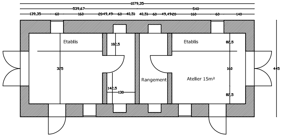
Plan 2 ateliers
